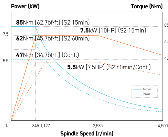
SE2600SY/LSY : Sub 4,500 rpm
