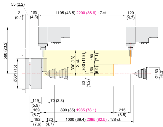
Axial driven
