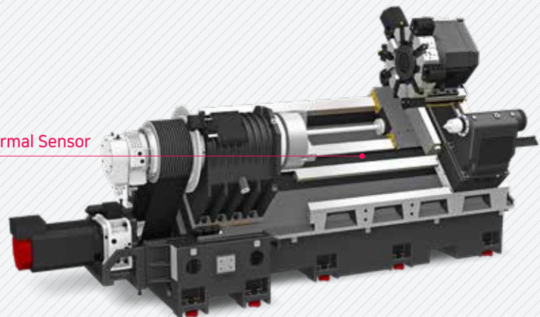
Structure thermal displacement error correction
