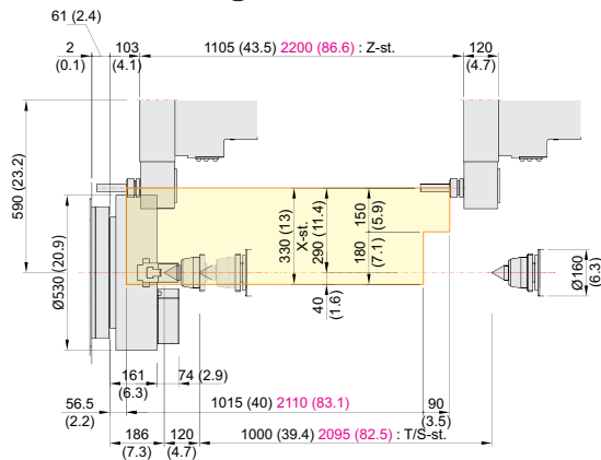
Angular driven
