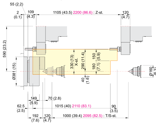
Angular driven
