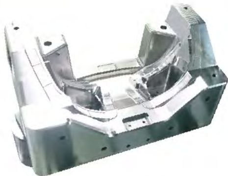
Automobile injection mold Material : Die steel Feature : 1. 5-axes tilting fixed aix rapping machining on recessed angle. 2. Uncoaxiality 5-axes machining, within tolerance.
