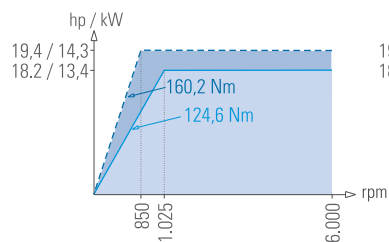
Headstock ASA A2-5" - 6,000 rpm
