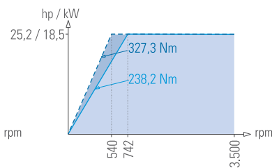
Headstock ASA A2-8" - 3,500 rpm
