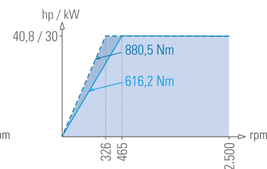
Headstock ASA A2-11" - 2,500 rpm
