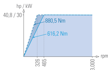
Headstock ASA A2-8" - 3,000 rpm
