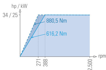
Headstock ASA A2-11" - 2,500 rpm
