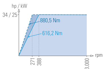
Headstock ASA A2-8" - 3,000 rpm
