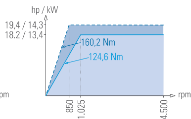
Headstock ASA A2-6" - 4,500 rpm
